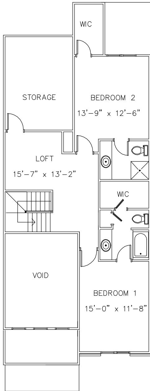
SECOND FLOOR
